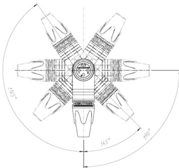
Outlet Positions
